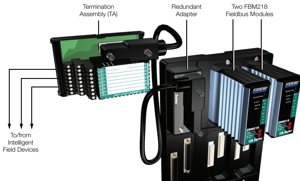
Figure 1. Redundant Module Configuration
